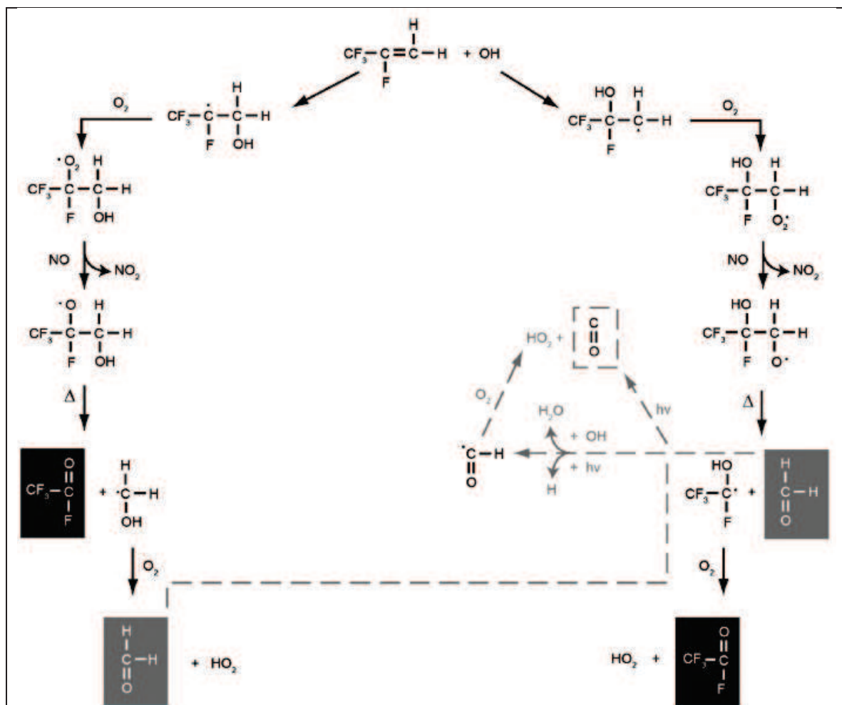
Figure 5-1: Atmospheric degradation mechanism for HFO-1234yf
