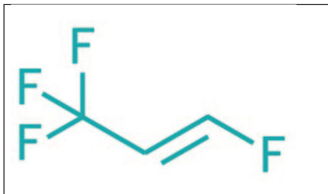
Figure 3-2: Structure of HFO-1234ze
