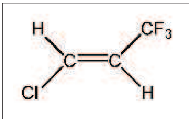
Figure 3-3: Structure of HFO-1233zd
