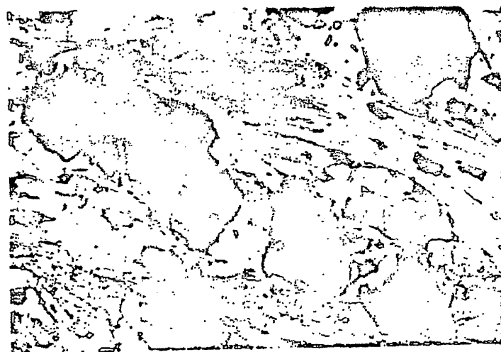
Fig. 15b Photomicrograph, x 24 mag., of thin section I 17 under XN. Garnet (black), quartz (white to grey), and muscovite (lamellar and coloured).
