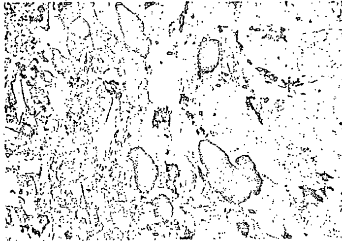
Fig. 10a Photomicrograph, x 40 mag., of thin section I13 under PPL showing subhedral pyrite meta-crysts (black) in a matrix of dominantly chlorite and quartz with minor calcite.
