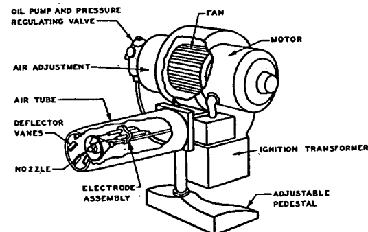
FIG. 12. HIGH-PRESSURE ATOMIZING OIL BURNER
