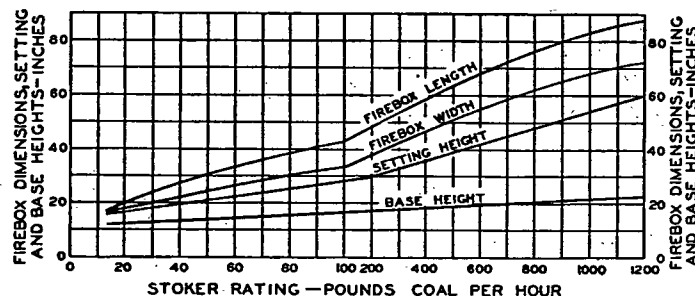
FIG. 11. SUGGESTED MINIMUM FIREBOX DIMENSIONS AND BASE HEIGHTS*
