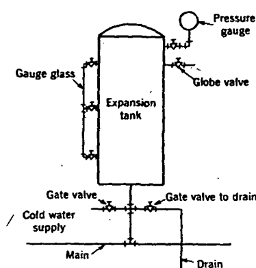
FIG. 10. A CLOSED EXPANSION TANK
