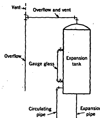
FIG. 9. AN OPEN EXPANSION TANK
