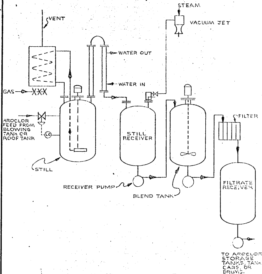
AROCLOR STILL-FLOW SHEET
