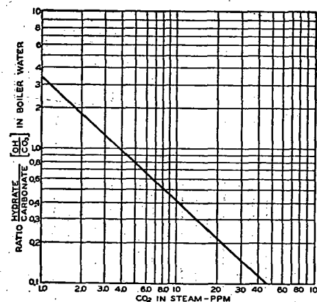
FIG. 5. RELATION OF HYDRATE/CARBONATE CONTENT IN Hard BOILER WATER AND CO 2 IN STEAM AT ABOUT 5 PSI OPERATING PRESSURE (All analytical values are ppm by weight)
