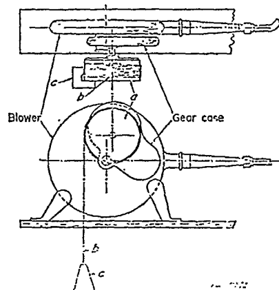
Figure 1.—Apparatus for measuring power required to operate blower. (39 CFR Part 11, Subpart J, § 11.124-3)
