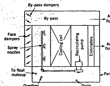
FIG. 11. RECIRCULATING SPRAY SYSTEM FOR CLEANING COILS
