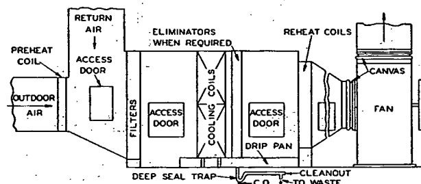
FIG. 9. TYPICAL ARRANGEMENT OF COOLING COILS IN A CENTRAL SYSTEM
