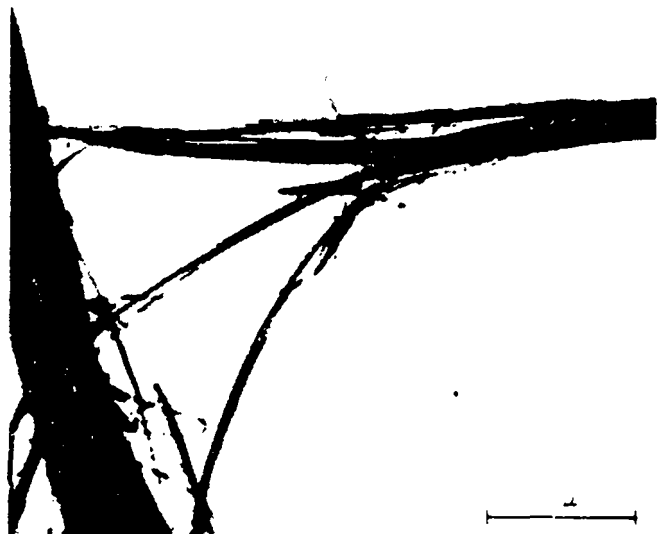
Fig. 5 - TEM image of partially opened fiber bundles
