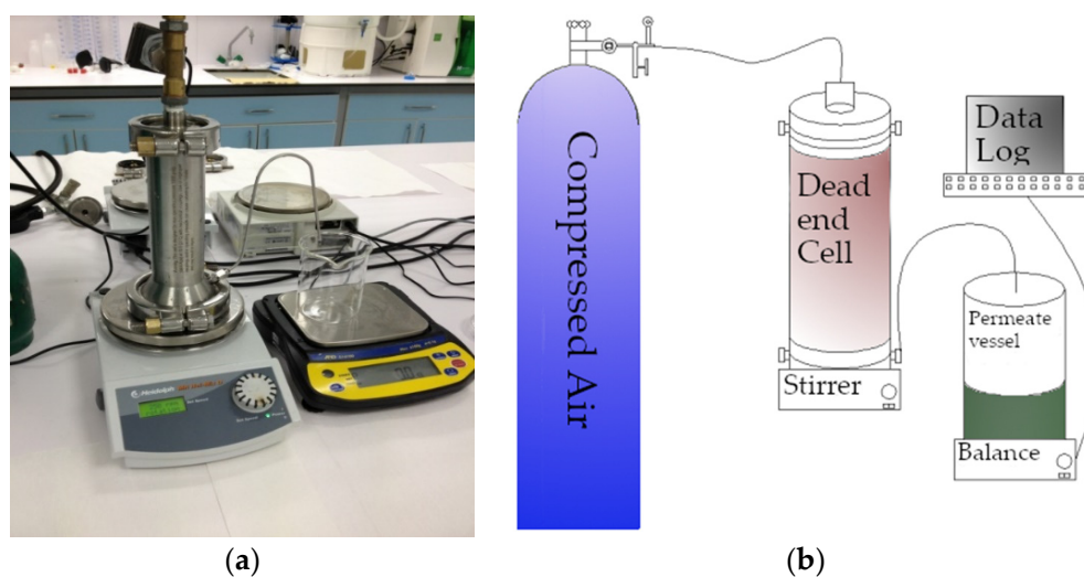
Figure 3. View of permeability test (a) experimental set-up (b) schematic diagram.
