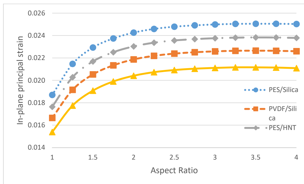
Figure 19. The maximum in-plane principal strain of nanocomposite membranes with different aspect ratios.
