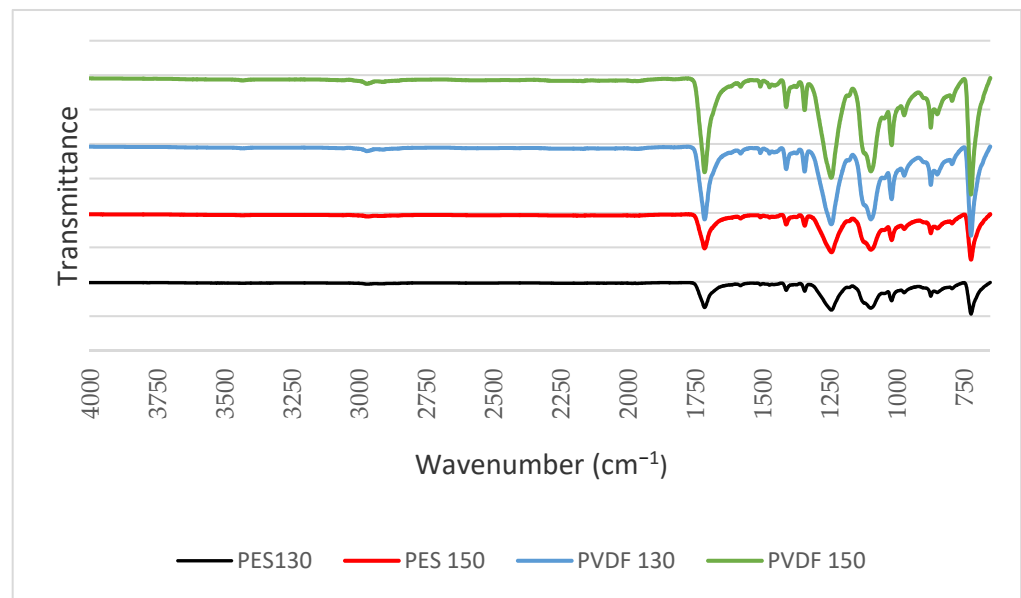
Figure 5. FTIR spectra of PES and PVDF membranes.
