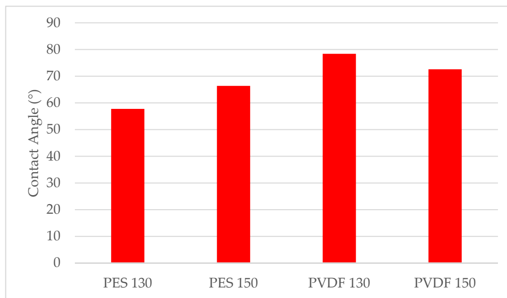
Figure 7. Membrane surface contact angles in degrees.
