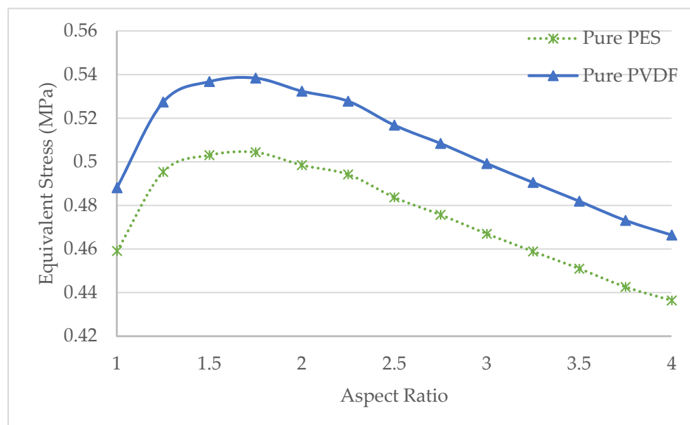
Figure 14. Maximum equivalent stresses of pure membranes of different aspect ratios.
