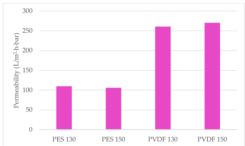
Figure 10. Permeability of membranes.
