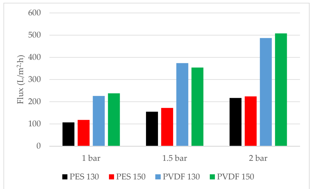
Figure 9. Flux values of membranes at different pressures.
