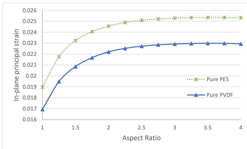
Figure 16. The maximum in-plane principal strain of pure membranes with different aspect ratios.
