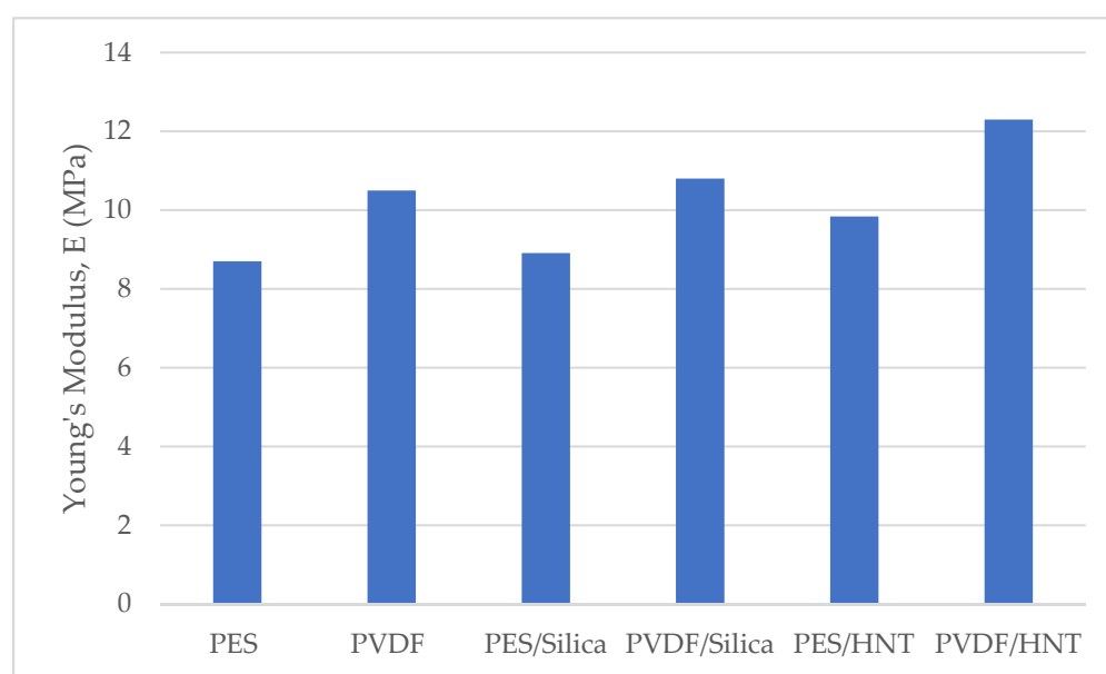
Figure 12. Young's modulus of pure and nanocomposite membranes.
