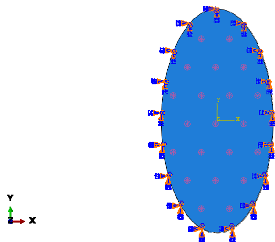
Figure 4. Boundary conditions and loads in the finite element model.
