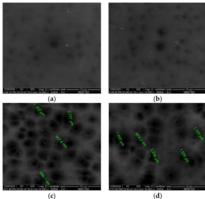
Figure 6. SEM surface images of membranes (a) PES 130, (b) PES 150, (c) PVDF 130, and (d) PVDF 150.
