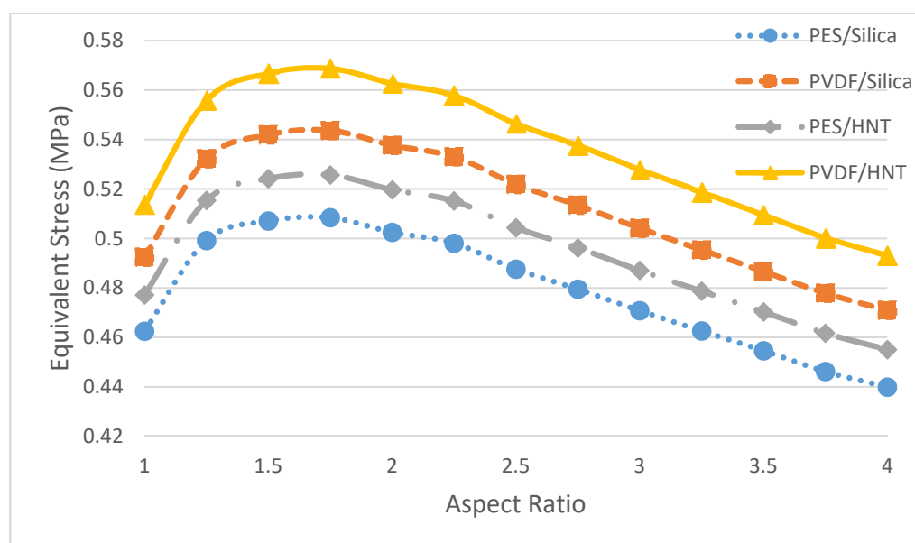
Figure 17. Maximum equivalent stresses of nanocomposite membranes of different aspect ratios.
