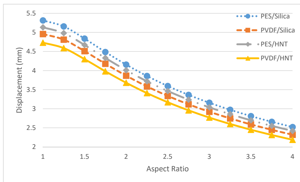
Figure 18. Maximum displacements of nanocomposite membranes with different aspect ratios.
