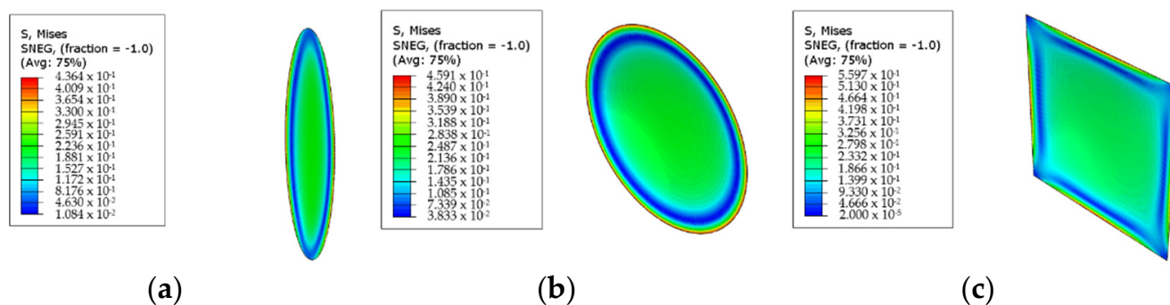
Figure 13. Visualised equivalent stress results of PES membranes: (a) ellipse 4 (b) circle (c) square membrane.
