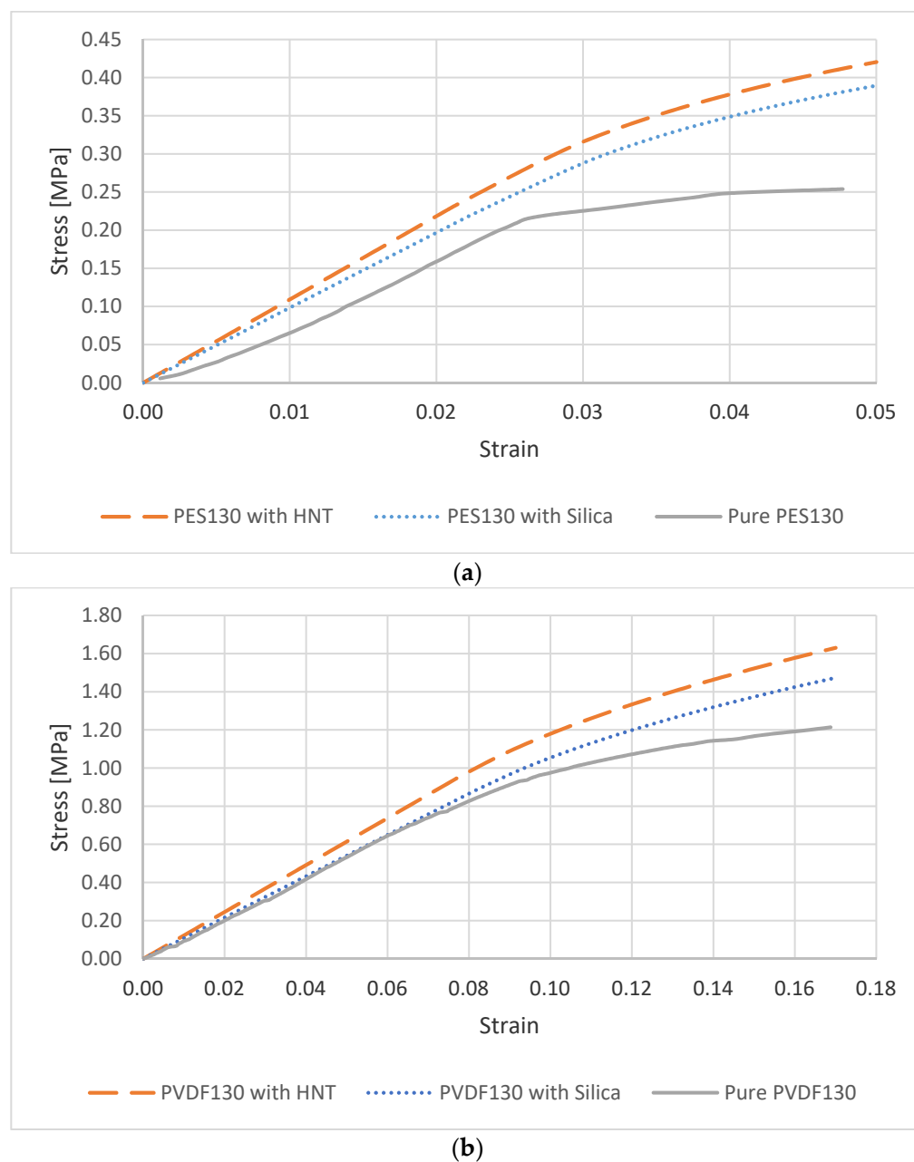
Figure 11. Stress-strain curves for the membranes (a) PES130 and its nanocomposites (b) PVDF130 and its nanocomposites.
