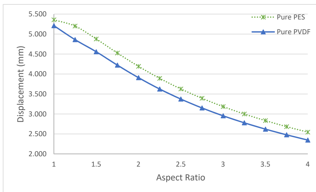
Figure 15. Maximum displacements of pure membranes with different aspect ratios.
