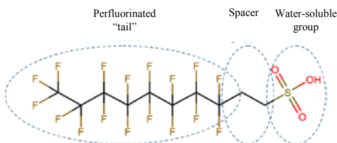
Figure 4: Schematic diagram of the formation of fluorosurfactants.
