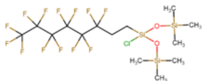
Trisiloxane, 3-chloro-1,1,5,5,5-hexamethyl-3-(3,3,4,4,5,5,6,6,7,7,8,8,8-tridecafluorooctyl)-
