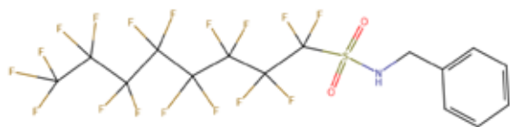
1-Octanesulfonamide, 1,1,2,2,3,3,4,4,5,5,6,6,7,7,8,8,8-heptadecafluoro-N-(phenylmethyl)-
