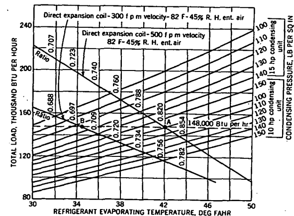
FIG. 10. COMPRESSOR AND COIL PERFORMANCE
