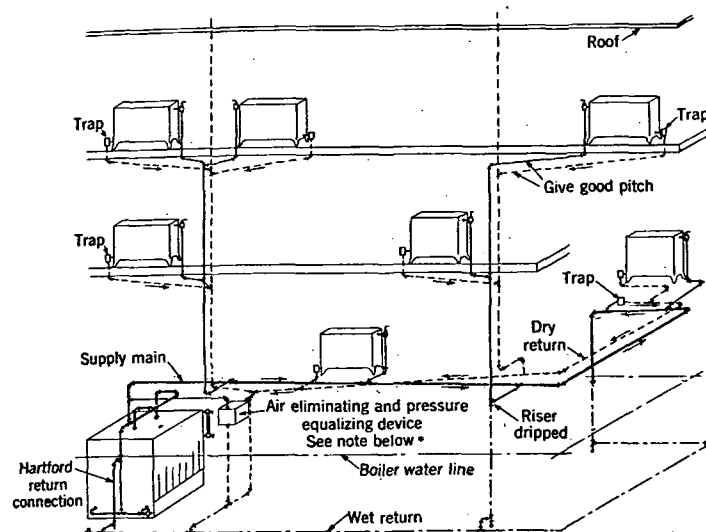
FIG. 13. TYPICAL ATMOSPHERIC SYSTEM WITH AUTOMATIC RETURN TRAPS a
