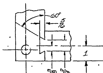
DETAIL A SCALE 6"=1"
