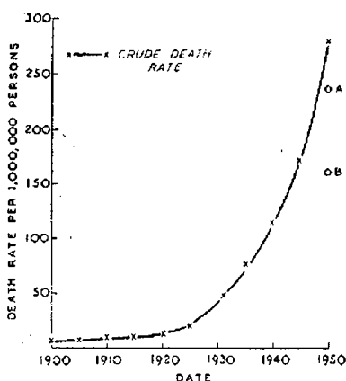
Fig. 2.—Death rate from lung cancer in England and Wales, 1900-50. A=Estimated death rate in 1950 with population of age and sex distribution as in 1931. B=Estimated death rate in 1950 with population of age and sex distribution as in 1901.
