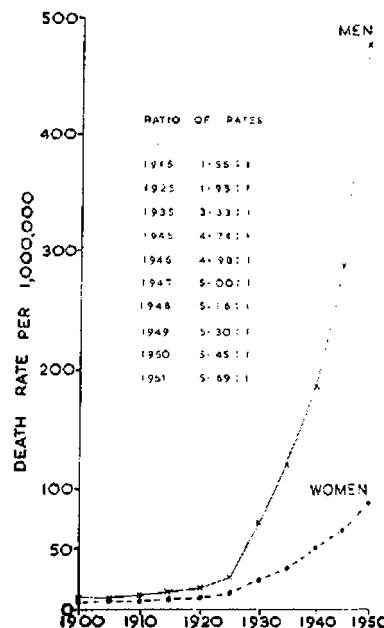
Fig. 3.—Death rates from lung cancer in England and Wales, 1900-50.
