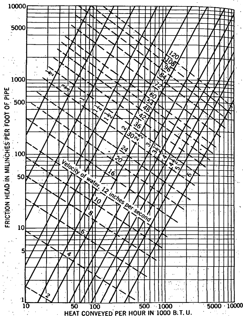
FIG. 4. FRICTION HEADS IN BLACK IRON PIPES FOR A 20 F TEMPERATURE DIFFERENCE OF THE WATER IN THE FLOW AND RETURN LINES
