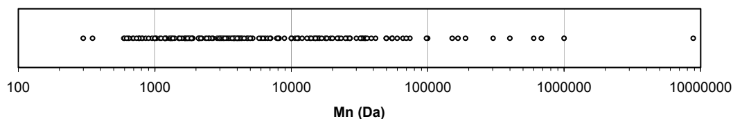
Figure 3. The distribution of Mn values in the dataset.
