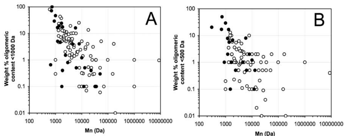
Figure 16. The relationship between M_n , oligomer content and health concern. (A) <1000 Da and (B) <500 Da oligomer content data. The low health concern polymers are represented by open circles (○), and the potential health concern by filled circles (●).
