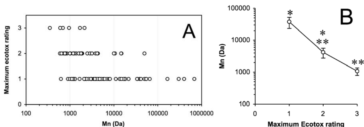
Figure 13. The influence of Mn on level of ecotoxicological concern. (A) The distribution of Mn data amongst polymers with each maximum ecotoxicological concern rating; (B) the average Mn value for each maximum ecotoxicological concern rating group. Error bars represent the standard error of each group; asterisks indicate statistical significance between data points (* p < 0.001 ; ** p < 0.05 ).
