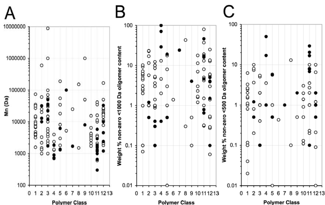
Figure 19. The distributions of Mn and oligomer content data in various polymer classes, for low and potential health concern polymers (represented by open (○) and filled circles (●), respectively). (A) Mn data; (B) <1000 Da and (C) <500 Da oligomer content. Only non-zero oligomer content data is represented.
