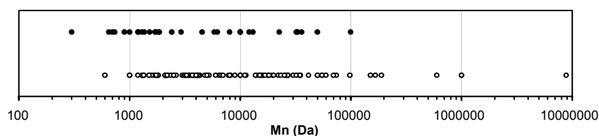
Figure 10. The distribution of Mn data amongst polymers with low and potential health concern ratings. The low health concern polymer dataset is represented by open circles (○), and the potential health concern dataset by filled circles (●).
