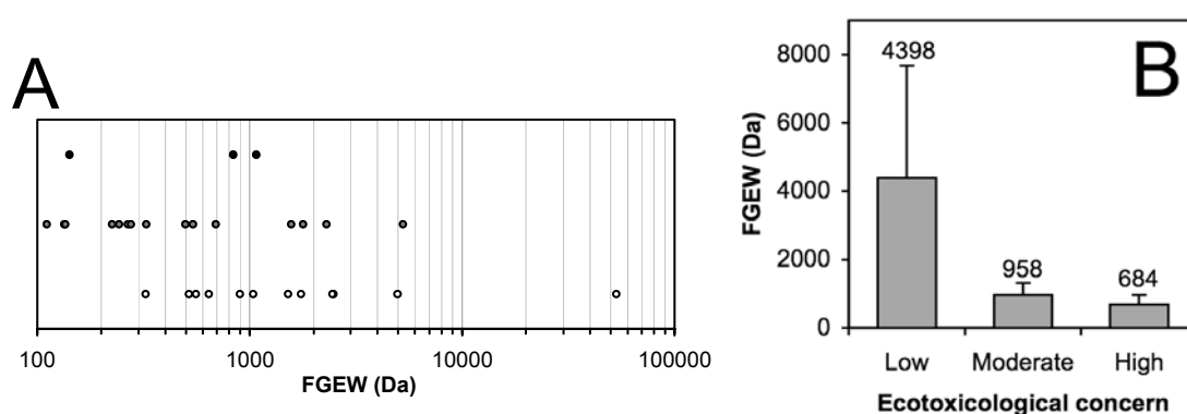
Figure 27. The relationship of FGEW and ecotoxicological concern. (A) The distribution of FGEW values in the ecotoxicological concern dataset, and (B) the average FGEW values within each level of ecotoxicological concern. The low ecotoxicological concern polymer dataset is represented by open circles (○), the moderate by grey-filled circles (●) and the high by black-filled circles (●). The error bars denote the standard error of each group.
