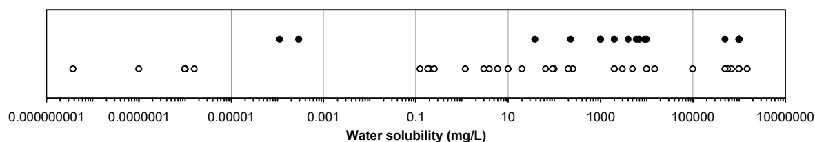
Figure 28. The distribution of water solubility data amongst polymers with low and potential health concern ratings (represented as open circles (○), and filled circles (●), respectively).
