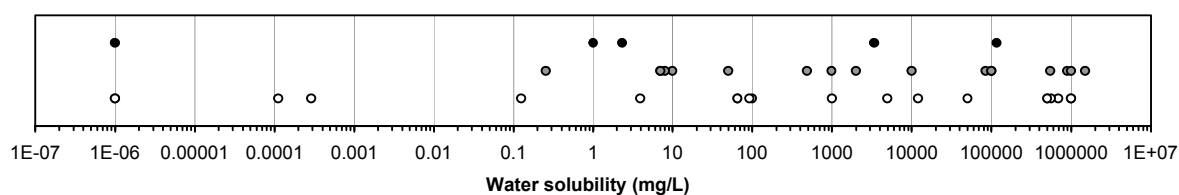
Figure 30. The distribution of water solubility data by ecotoxicological concern rating. The low ecotoxicological concern polymer dataset is represented by open circles (○, lower), moderate by grey-filled circles (●, middle) and high by black-filled circles (●, upper).
