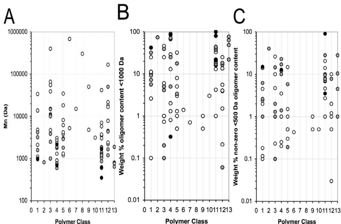
Figure 21. The relationship of Mn, oligomer content and polymer class on ecotoxicological concern. (A) Mn, (B) <1000 Da oligomer content and (C) <500 Da oligomer content. The low ecotoxicological concern polymer dataset is represented by open circles (○), moderate concern by grey-filled circles (●) and high concern by black-filled circles (●).
