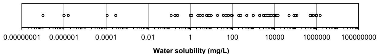
Figure 4. The distribution of water solubility/extractability data
