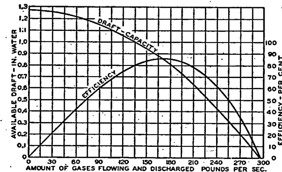
FIG. 2. TYPICAL SET OF OPERATING CHARACTERISTICS OF A NATURAL DRAFT CHIMNEY
