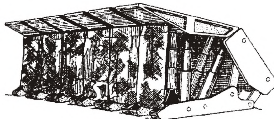
Figure 4. Mesh barrier hung from longwall supports (from Organiscak and Leon, 1993).
