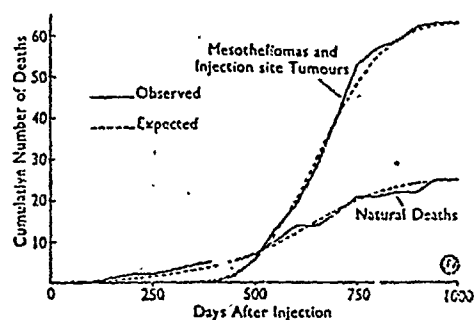
Fig. 2. Experiment A: Comparison of observed and expected distribution of deaths for crocidolite in Standard rats. The expected deaths are calculated from the model given in the text with a = -10.4 , b = 0.00586 , c = 1.54 \times 10^{-6} , k = 3 , w = 332 .
