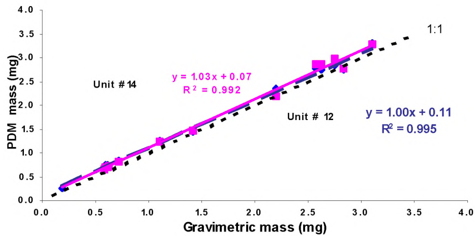
Figure 10. Longwall gallery regression using keystone coal
