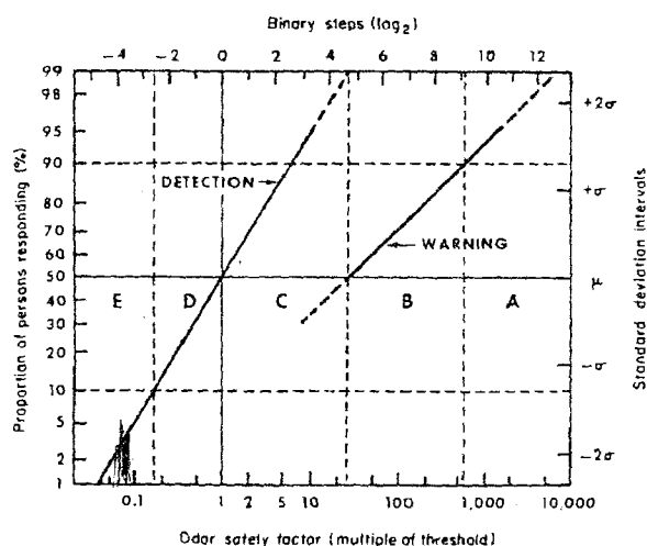
Figure 2. A practical guide to the quantitative interpretation of odor safety factors. The coordinates are log/probit, so care is required in interpolating between marked intervals. The sloping lines indicate the percentages of the population expected to respond to various fractions or multiples of the mean detection threshold concentration (1.0 on the x axis). The detection line represents the performance of fully attentive persons under good laboratory conditions. The warning line shows what may be expected for distracted persons under factory or field conditions. The warning line is based on the results of Whisman et al. 19 for the gas odorants ethyl mercaptan and thiophane.
