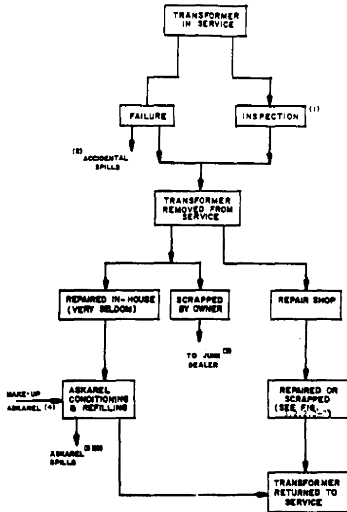
FIGURE 3.2.2.2-1. TRANSFORMER MAINTENANCE & SERVICING
