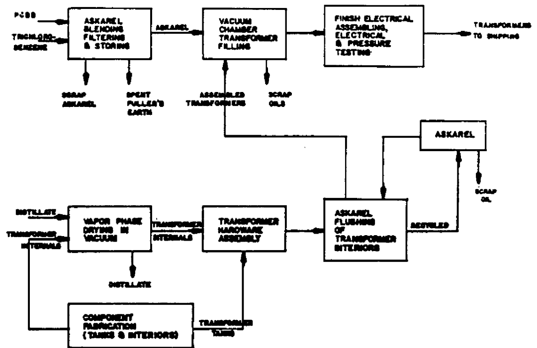
Figure 3.2.1.2.1-1 TRANSFORMER FILLING WITH VAPOR PHASE PREDRYING OF INTERIORS
