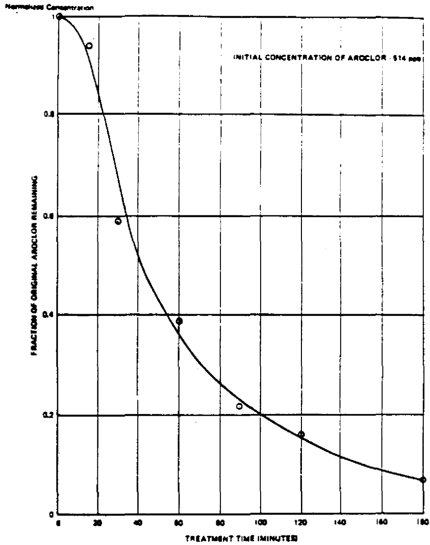
Figure 2.2.2.4.1-2. AROCLOR 1254 DESTRUCTION BY UV-ASSISTED OZONATION
