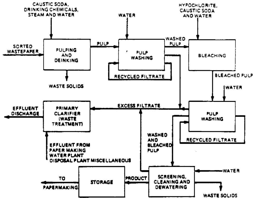
Figure 3.4.2-1. MILL FIBER RECOVERY PROCESS AND WATER EFFLUENTS
