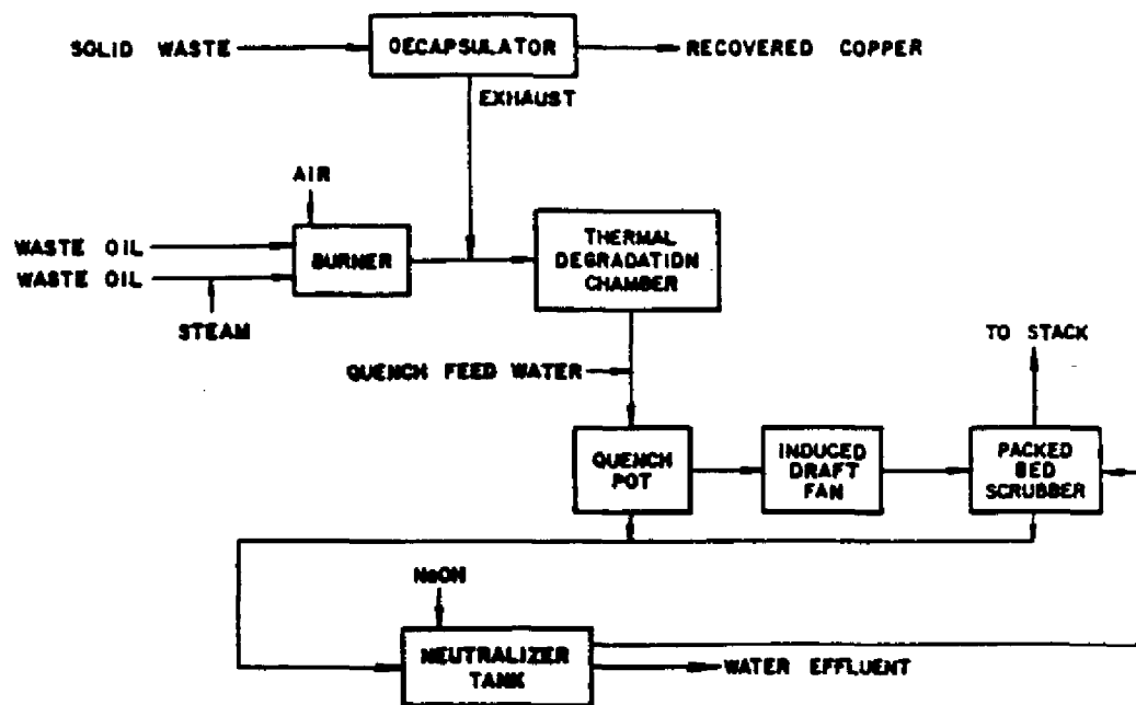
Figure 3.2.1.5-1. PROCESS FLOW DIAGRAM FOR THERMAL OXIDIZER INCINERATOR AT PLANT 103
