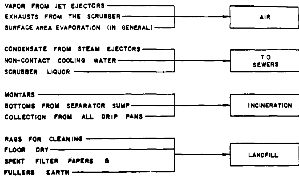
FIGURE 2.2-1. NON-PRODUCT PCB DISCHARGES AT MONSANTO'S KRUMMRICH PLANT
