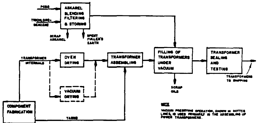
Figure 3.2.1.2.1-2 TRANSFORMER FILLING WITH OVEN OR VACUUM CHAMBER PREDRYING OF TRANSFORMER INTERNALS
