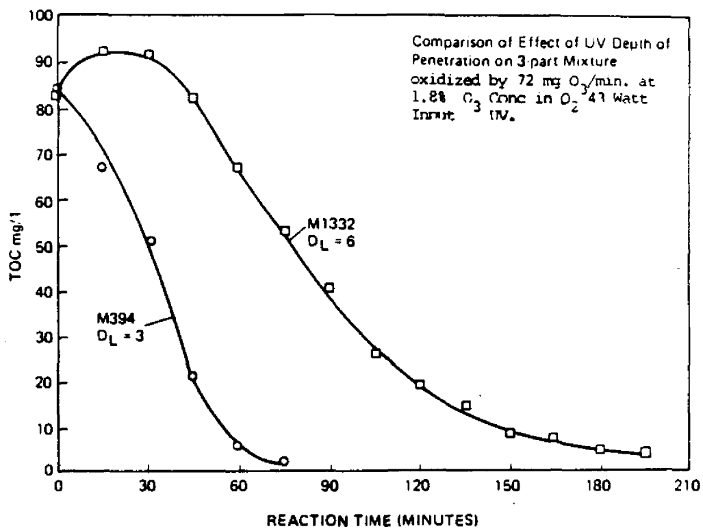
Figure 2.2.5.2-1. THE EFFECT OF UV PATH LENGTH ON TOC DESTRUCTION
