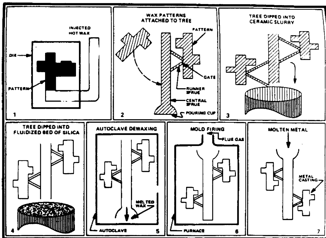
Figure 3.3.2.1-1. INVESTMENT SHELL PROCESS
