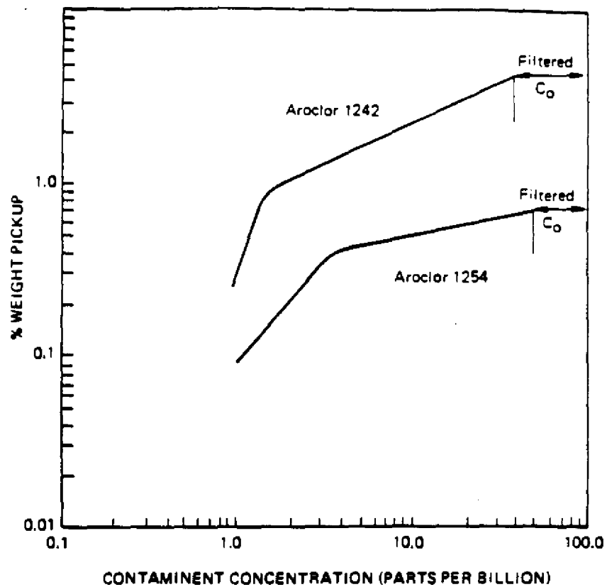
Figure 2.2.1.3-1. EQUILIBRIUM CARBON ADSORPTION OF PCB'S FROM WATER AT LOW CONCENTRATIONS (CALGON DATA)
