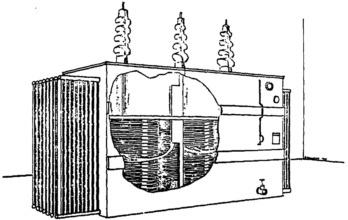
FIGURE 3.2.1-1. SUBSTATION TRANSFORMER
