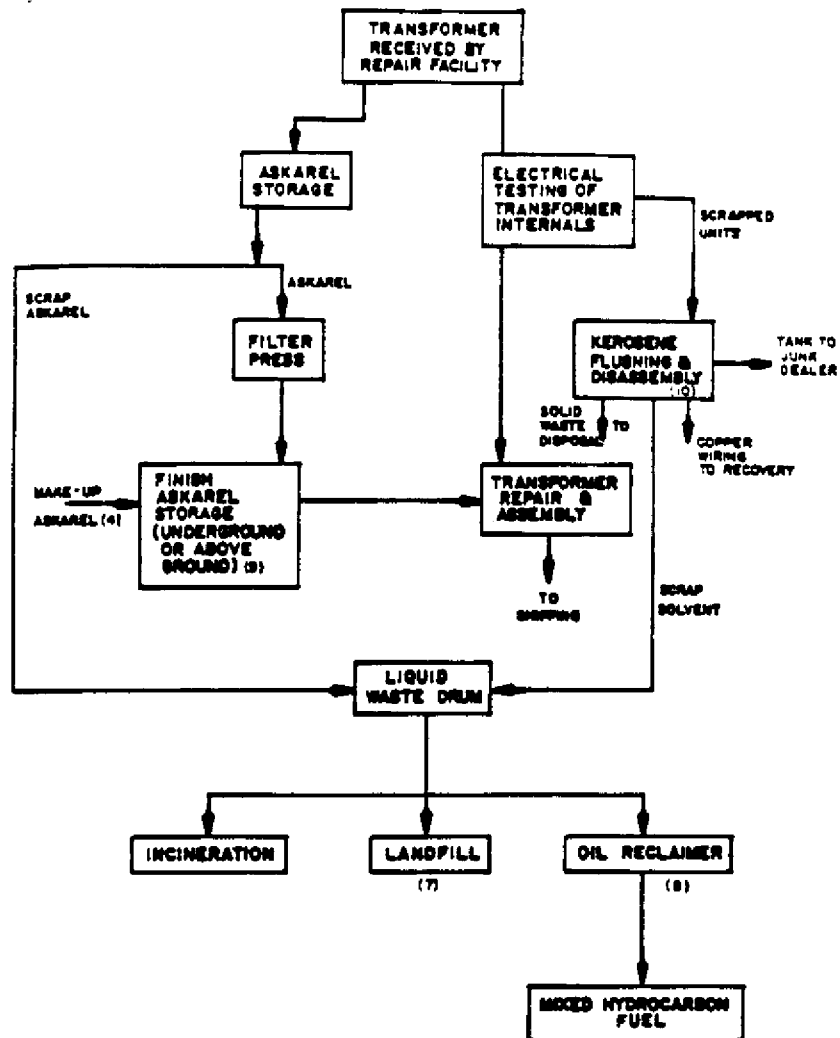
FIGURE 3.2.2.2-2. TRANSFORMER REPAIR
