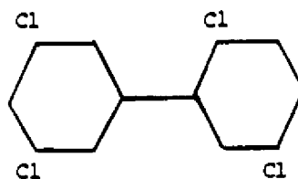
2,3',5,5'-tetrachlorobiphenyl
