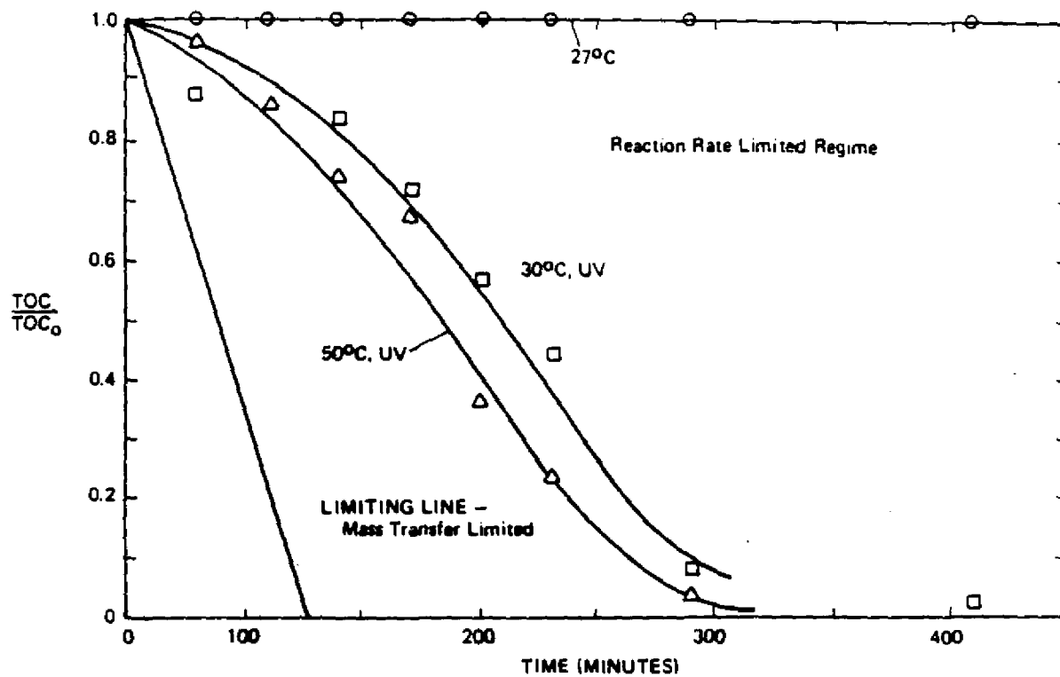
Figure 2.2.2.4.2-1. DZONE OXIDATION OF ACETIC ACID, EFFECT OF UV AND TEMPERATURE (INITIAL CH_3COOH - 106 mg/l, O_3(l) - 3.5 mg/l)
