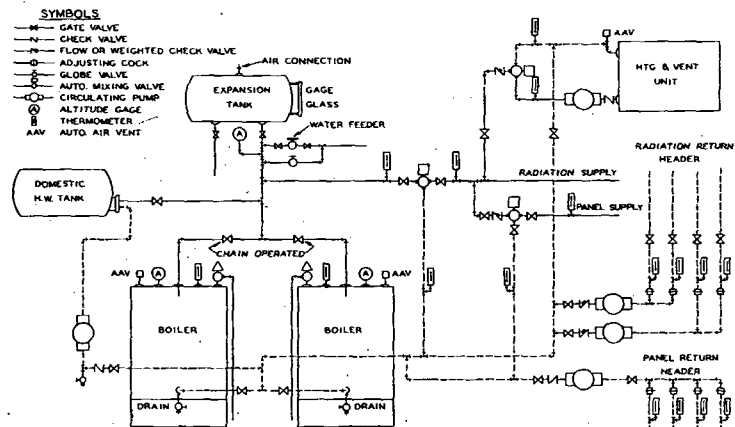
Fig. 19. . . . Boiler Piping for Multiple-Zone Multiple-Purpose Heating System
