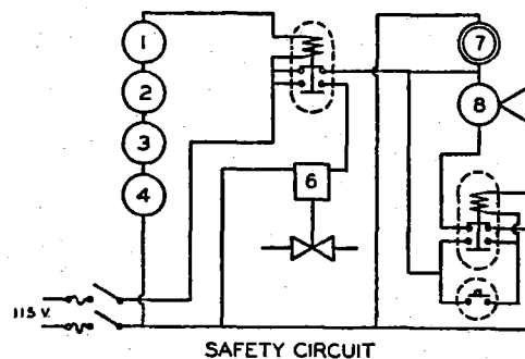
Figure 3. Control and Safety Circuit
