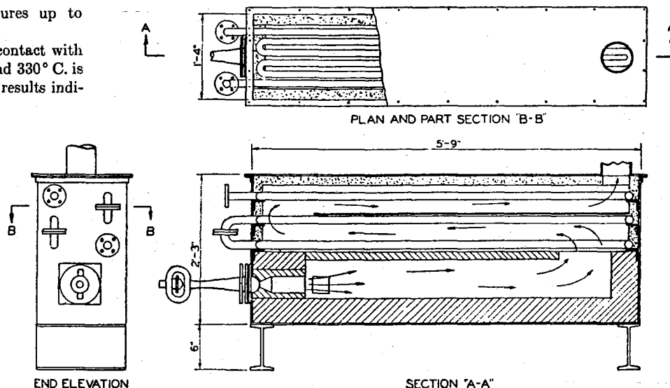
Figure 1. Heater
