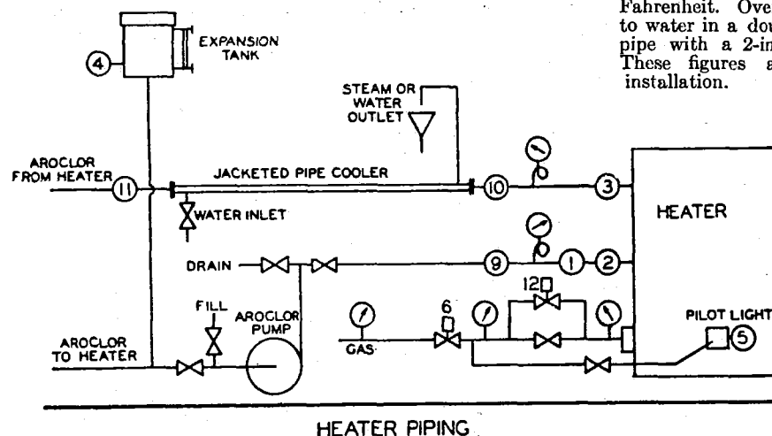
Figure 2. Cooler, Pump, and Expansion Tank
