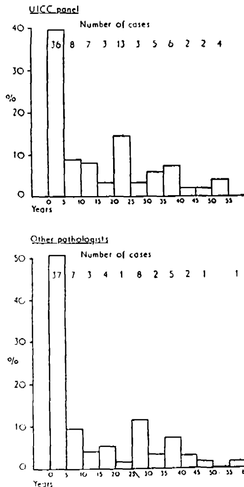
FIG. 3. Definite mesotheliomas with definite occupational asbestos exposure: survival after last exposure.
