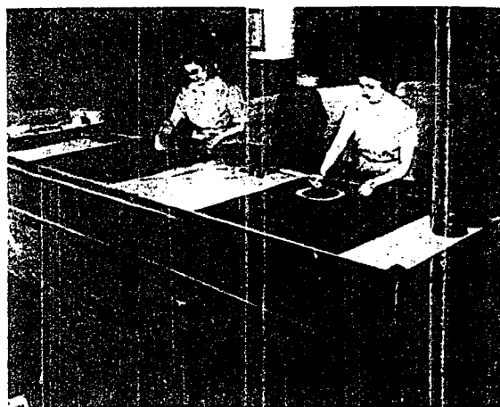
Control of solvent vapors by local exhaust ventilation (slot at edge of table top) at a fabric cementing operation.
