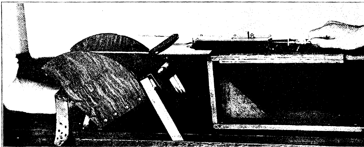
Fig. 2.—Apparatus for testing strength of flexor and extensor muscles in the forearm in use for testing the extensors of the left wrist. The pull is being exerted by the operator on the spring of the smaller recording dynamometer which rests on the roller carriage, while the hand of the subject being tested, palm downward, is in the nest for the whole hand with the axis of rotation of the wrist kept in line with the axis of the wooden pulleys; the subject endeavors to prevent the index on the tilting platform from falling below the point marked 22^{\circ} 30' on the brass scale.
