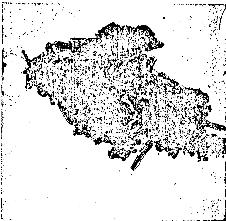
FIG. 7. Electron photomicrograph of air sample taken during brake drum blowing (see sample No. 4, Table 5). Large numbers (70-100) of chrysotile, some of which are masked by granular particulates, presumably road dust (65,000 total magnification).
