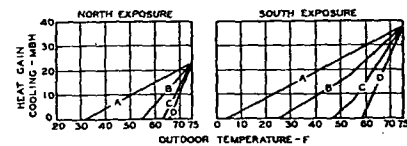
Basic Cooling requirements shown in Fig. 1. A = Net heat gain with ventilation air controlled at room temperature of 75°F. B, C, and D = Net heat gain using 525, 1000, and 1500 cfm, respectively, controlled to 55°F, minimum. Cooling air temperature will be higher as outdoor air temperature rises above 55°F.
