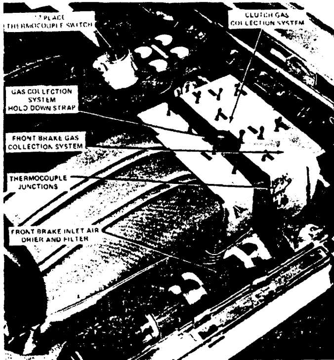
Fig. 2 - Vehicle instrumentation (front seat area)
