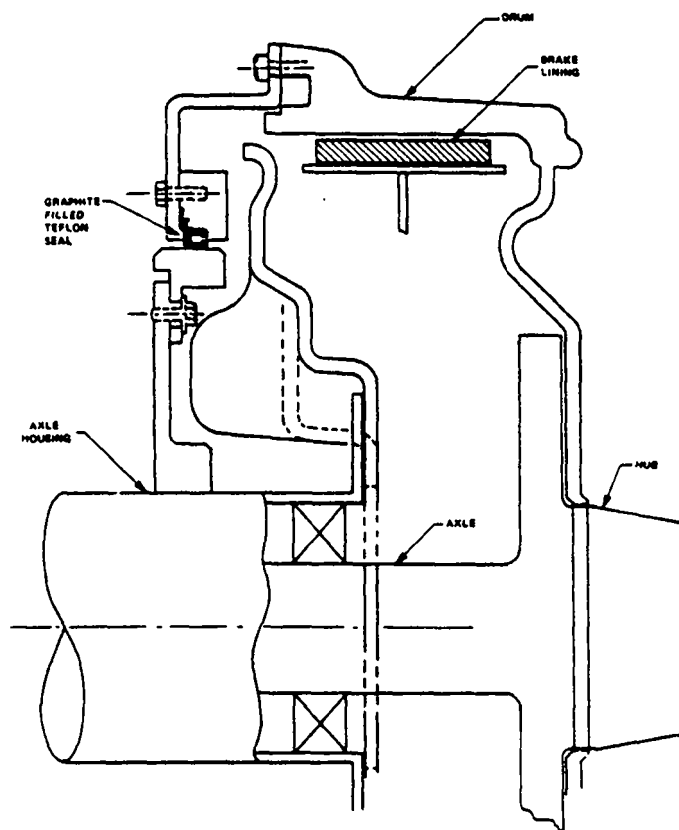
Fig. 8 - Schematic of drum brake shroud
