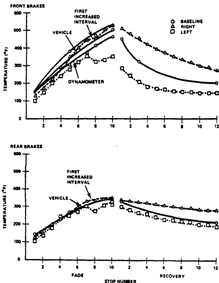
Fig. 12 - Brake temperature data during 10 Stop Fade Test
