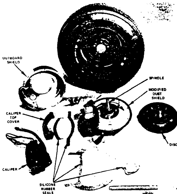
Fig. 5 - Disc brake emissions collector assembly—exploded view
