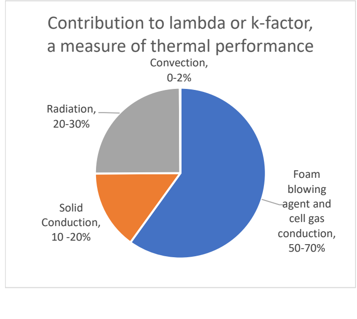
Figure 2.25 Importance of FBA to XPS thermal performance by reducing heat transfer through gas conduction.
