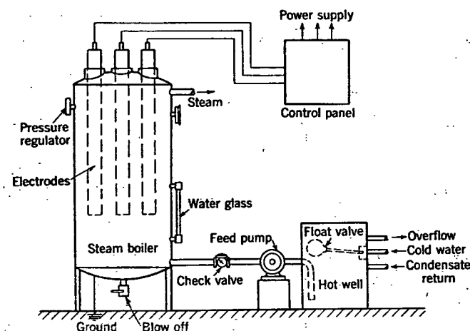
FIG. 3. DIAGRAMMATIC ARRANGEMENT OF AN ELECTRODE BOILER
