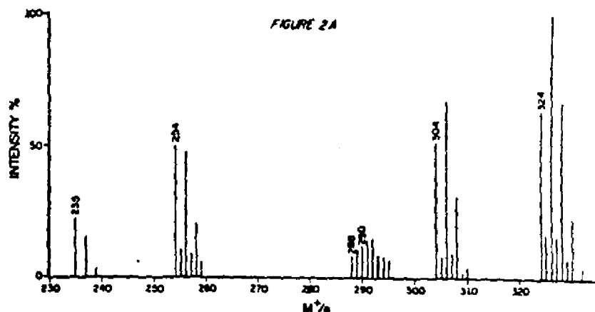
Figure 2A Mass spectrum resulting from GC-MS analysis of 88 mls of rat urine. LKB 9000 GC-MS, mass marker \pm 0.3 mass unit. GC column temperature, 209°C; flash heater 235°C; glass coiled column, 6'x1/4" 1.5 OV-17/1.95 QF-1 on 60/80 mesh chromosorb "W" H.P., A.W., DMCS; carrier gas (He) 30 psi and 45 cc/min.; separator, 320°C; source 290°C; energy, 70 eV; accelerating voltage, 3.5 KV; trap current, 60 uA; box current, 50 uA; leak current, 8 uA.
