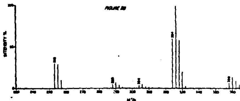
Figure 2B Mass spectrum resulting from GC-MS analysis of Fraction V 25% Et 2 O/Hex of Aroclor 1254 ® . LKB 9000 GC-MS, other conditions see fig. 2A. Instrument calibrated with PTK.
