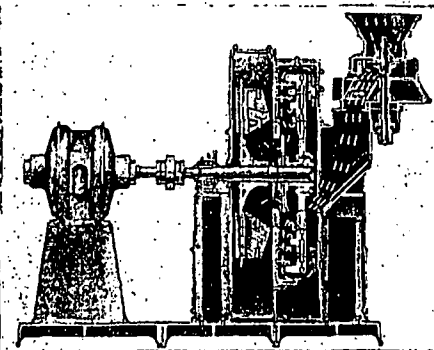
Riley Atrita Unit Pulverizer
