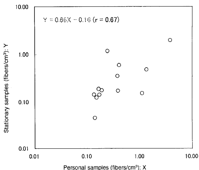
Figure 5—Relationship between geometric mean asbestos concentrations of personal and stationary samples at 13 unit work areas.
