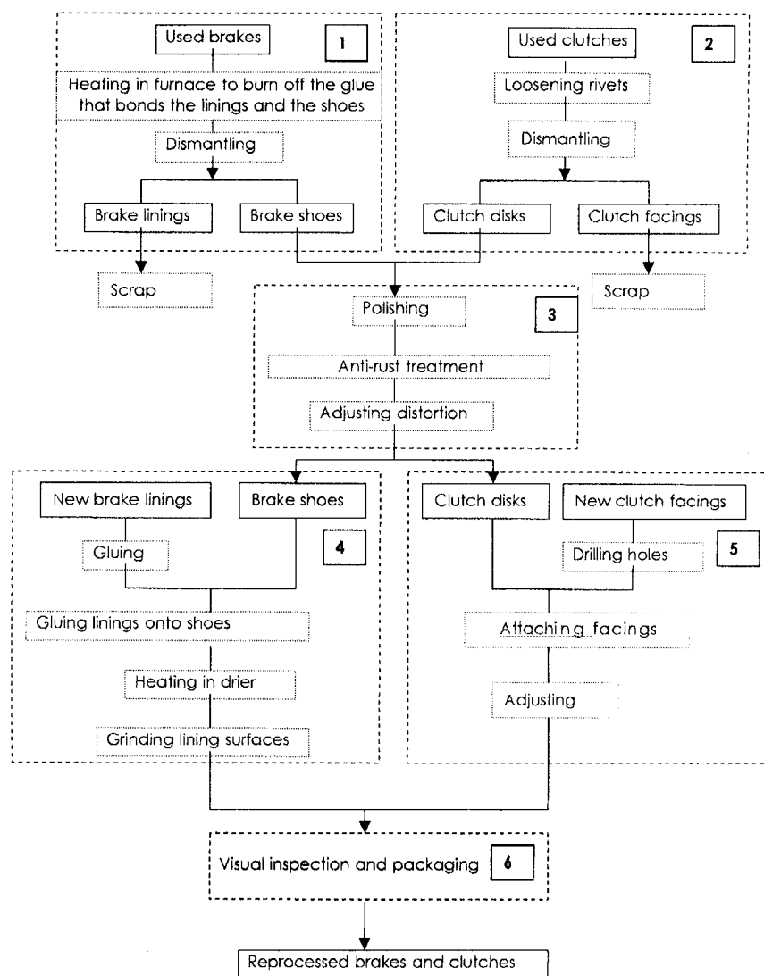
Figure 1—Sequence of operations in the reprocessing of brakes and clutches. Boxed numbers indicate process numbers in Table 3.
