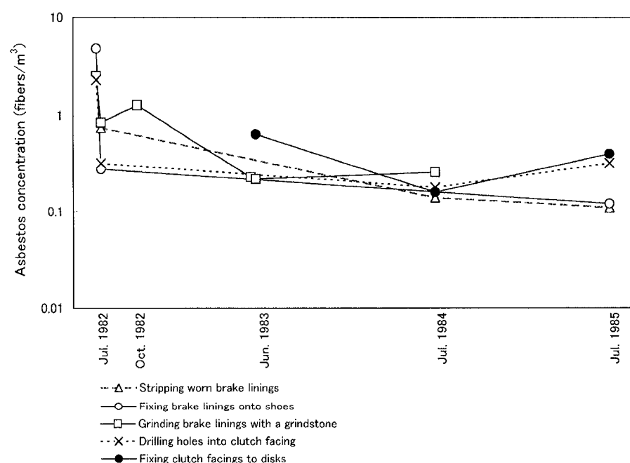
Figure 3—Trends of geometric mean asbestos concentrations from 1982 to 1985 in personal samples classified by operations in factory A.
