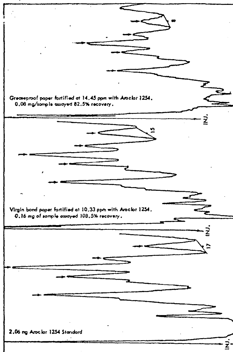
Figure 2 - REPRESENTATIVE CHROMATOGRAMS OF A 1254, AROCLOR AND FORTIFIED PAPERBOARD SAMPLES.
