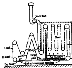
FIG. 5. SMALL PART MULTIPLE PASS OVEN
