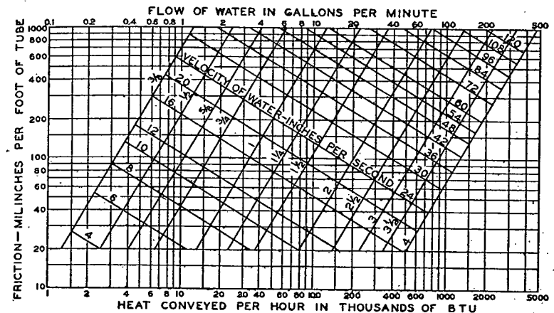
FIG. 3. FRICTION IN TYPE L COPPER TUBING
