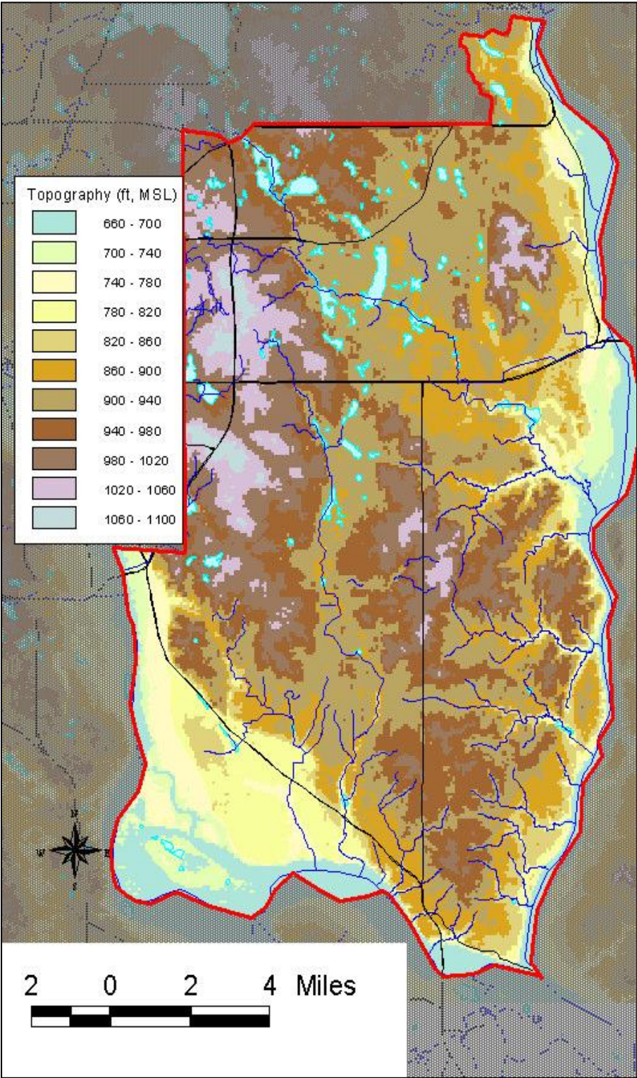
Figure 3 Ground-Surface Topography (feet, MSL)
