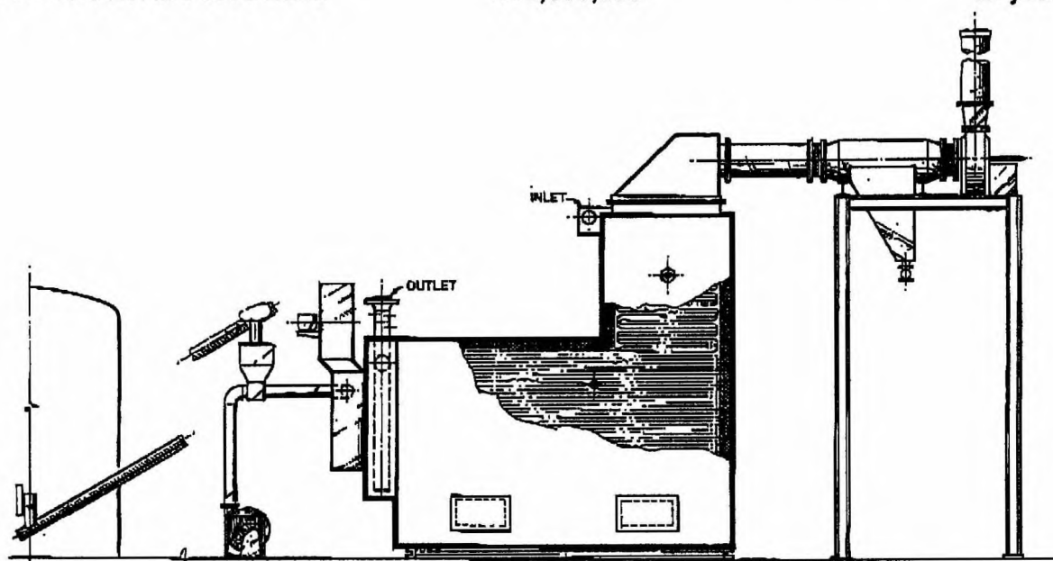
Fig. No. 5 - Suspension Fired
