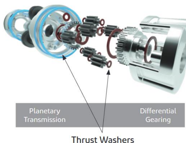
Figure 12: Illustration of thrust washers.
