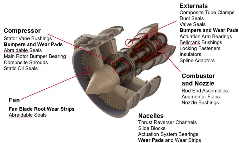
Figure 13: Vespel® components used within aircraft engine manufacturing.
