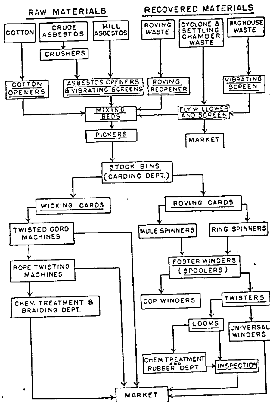
FIGURE 1.—Process flow sheet, asbestos textile plant.
