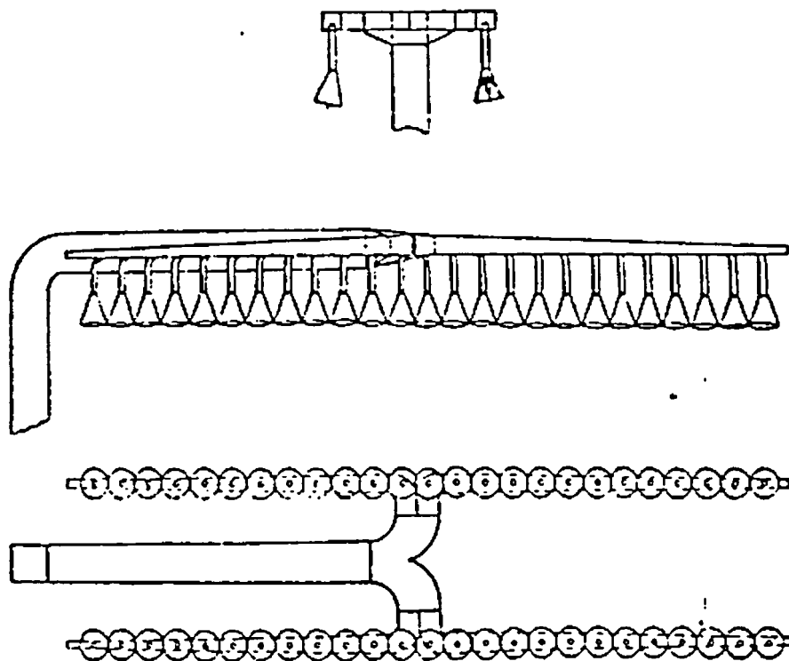
FIGURE 1 -- Schematic views of exhaust system applied to Foster winders
