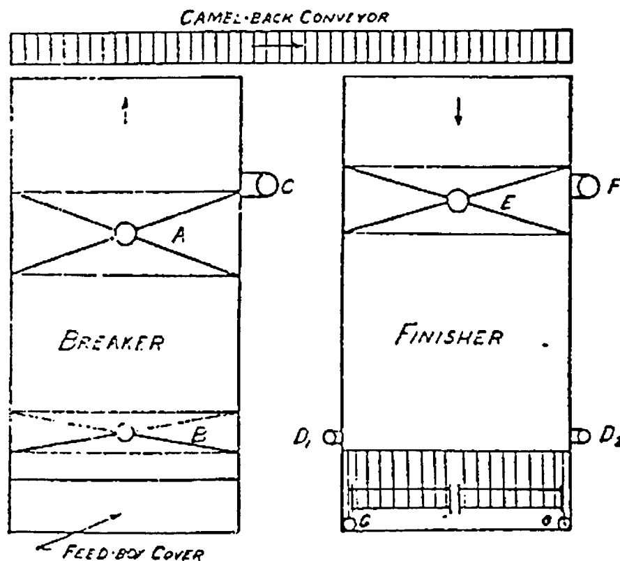
FIGURE 7—Schematic plan of card exhaust system
