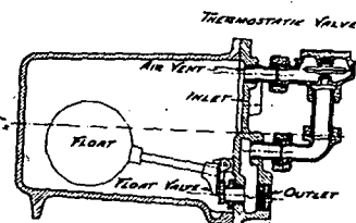
Sectional Detail of Blast Trap No. 16
