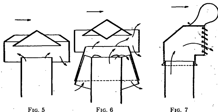
VARIOUS STYLES OF ROOF VENTILATORS
