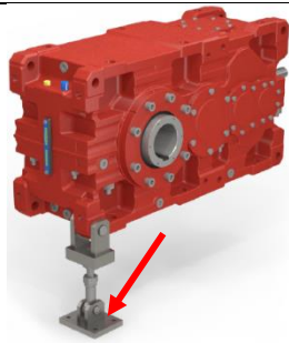
Figure 7: Joint head in the torque arm of an industrial gear unit (left) and in an electric cylinder (right) © SEW-EURODRIVE GmbH & Co KG
