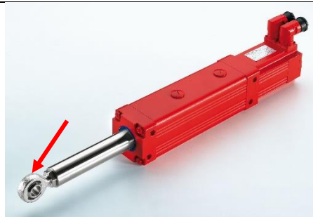
Figure 7: Joint head in the torque arm of an industrial gear unit (left) and in an electric cylinder (right) © SEW-EURODRIVE GmbH & Co KG
