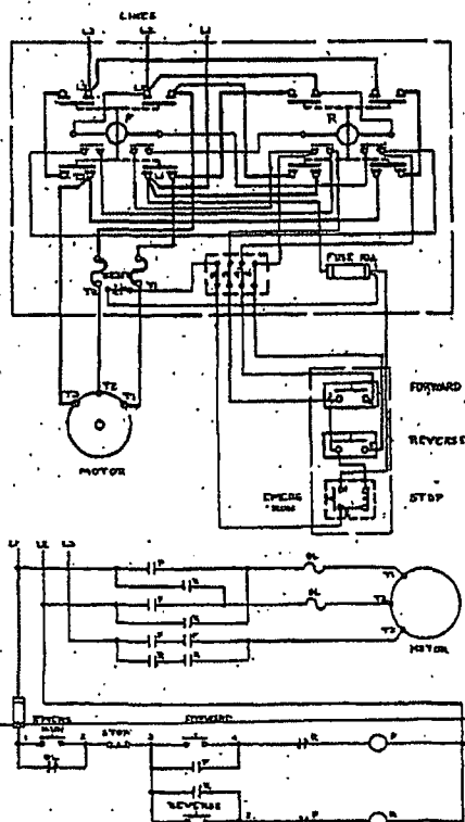
FIGURE 3 Size 1 and 2 reversing controllers providing overload and low voltage protection with remote master station, including emergency run.
