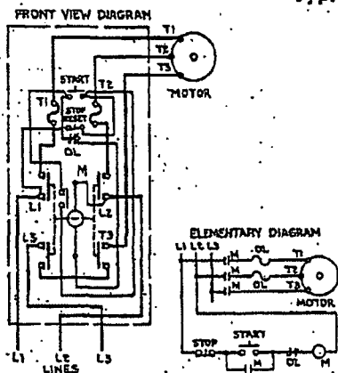
FIGURE 1 Size 1 and 2 non-reversing starters providing overload and low voltage protection, with local "start-stop" control.
