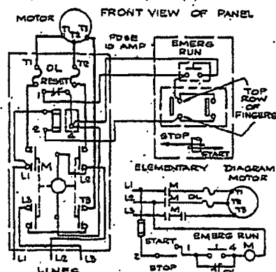
FIGURE 2 Size 1 and 2 non-reversing starters providing overload protection and low voltage release with remote master station, including emergency run feature.
