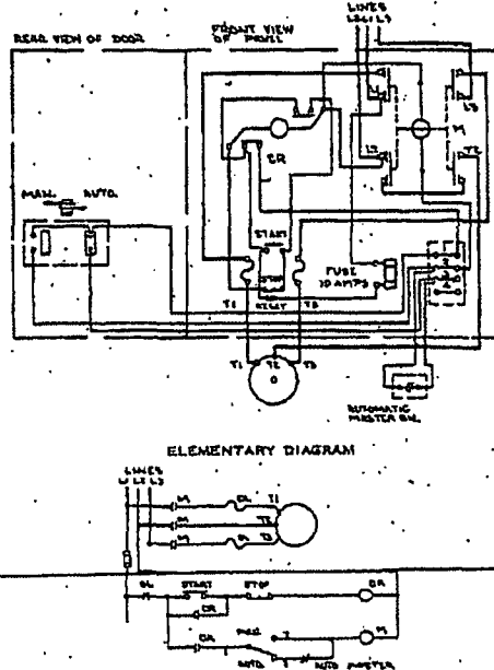
FIGURE 4 Size 1 and 2 non-reversing starters with control relay providing overload and low voltage protection, with local master station and remote automatic pilot master switch.
