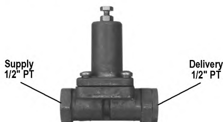
SC-PR Single Check Protection Valve – must be used in conjunction with the AD-SP Air Dryer 065677 - Service New 5000148X - Reman
