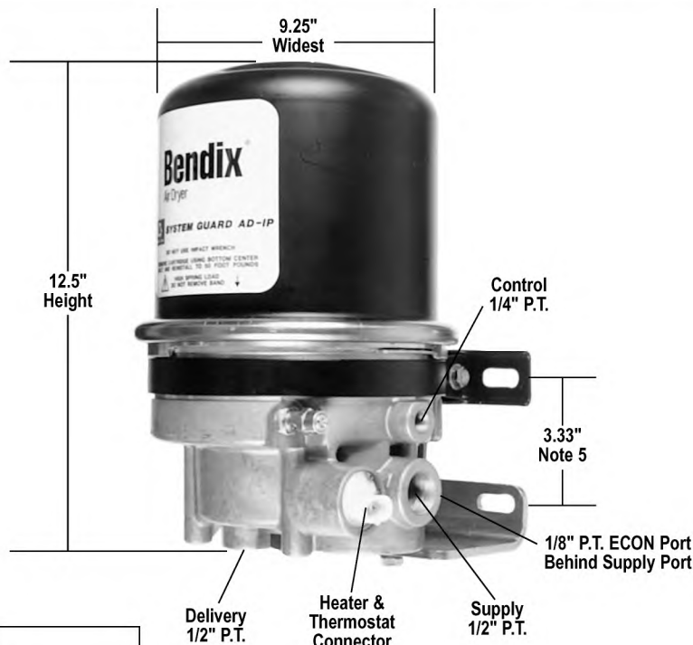
Extended Purge Kit 5005309
