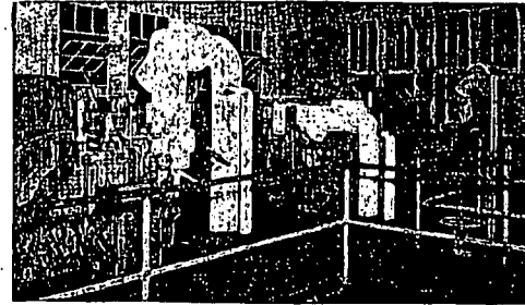
Above cut shows our 2250 KVA. General Electric Condensing Marine Type Turbine Generator. A Complete Machine with Condenser.
