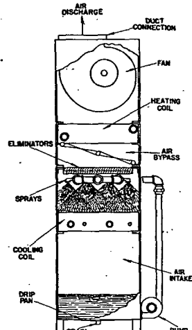
FIG. 16. SPRAY TYPE AIR CONDITIONING UNIT
