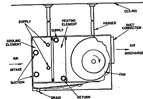
FIG. 17. HORIZONTAL REMOTE TYPE ALL-YEAR-ROUND CONDITIONING UNIT
