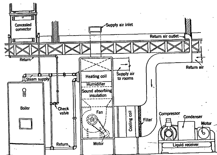
FIG. 18. RESIDENTIAL CONDITIONING UNIT WITH STEAM BOILER
